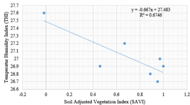
Figure 3. The regression equation between SAVI with THI
