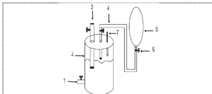
Figure 1. Schematic process of biodigester in laboratory scale: 1. Outlet; 2. Biodigester; 3. Inlet of raw materials; 4. Biogas hose; 5. Biogas shelter; 6. Control valve; and 7. Thermometer.
